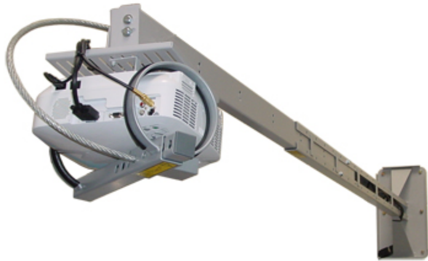
Extendable boom shown with optional n-circle security clamp and heavy duty cable kit.
